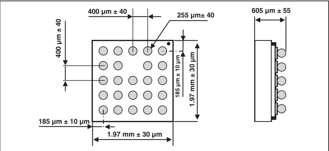
Figure 12. Package dimensions
